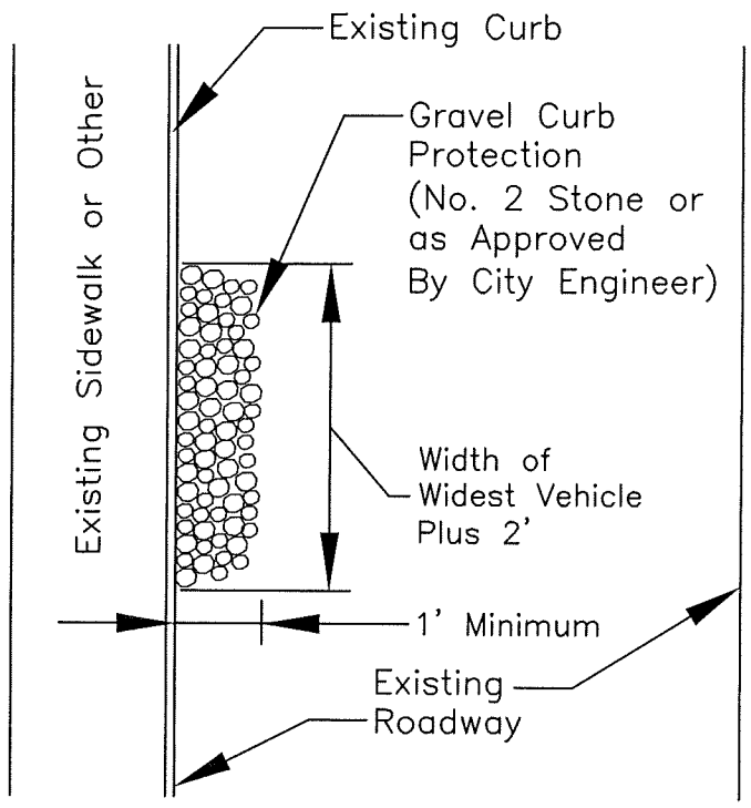
PLAN VIEW
